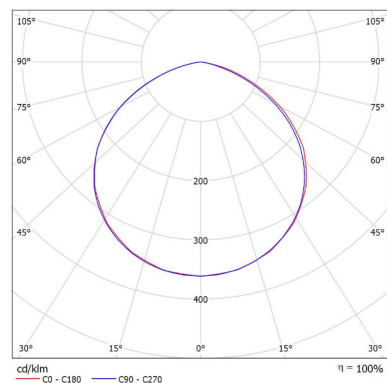
Luminaire: ADDIS Q-COMPACT AHC070WBL30C850 Lampes: 1 x PH3030-5000K-CRI80
