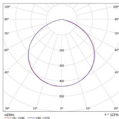
Luminaire: ADDIS Q-COMPACT AHC070WBL30F840 Lampes: 1 x PH3030-5000K-CRI80
