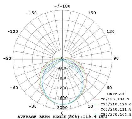
Cône de performance ABE15T54WC850
