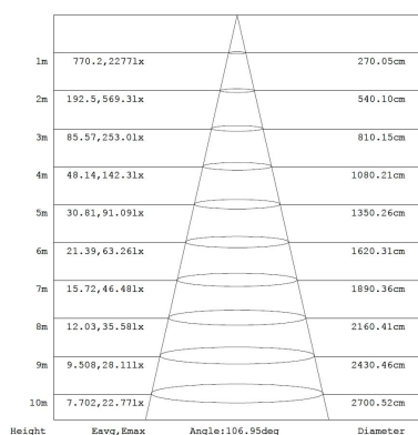
Cône de performance ABE15T54WC850
